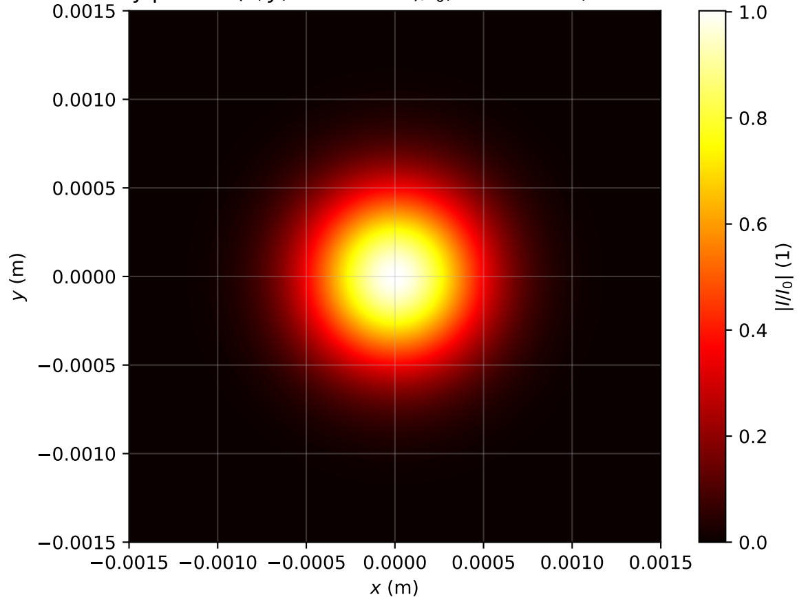
Intensity profile I(x, y, z = 0.239m)/I_0 , Pin=0.3Pcr, artificial time
